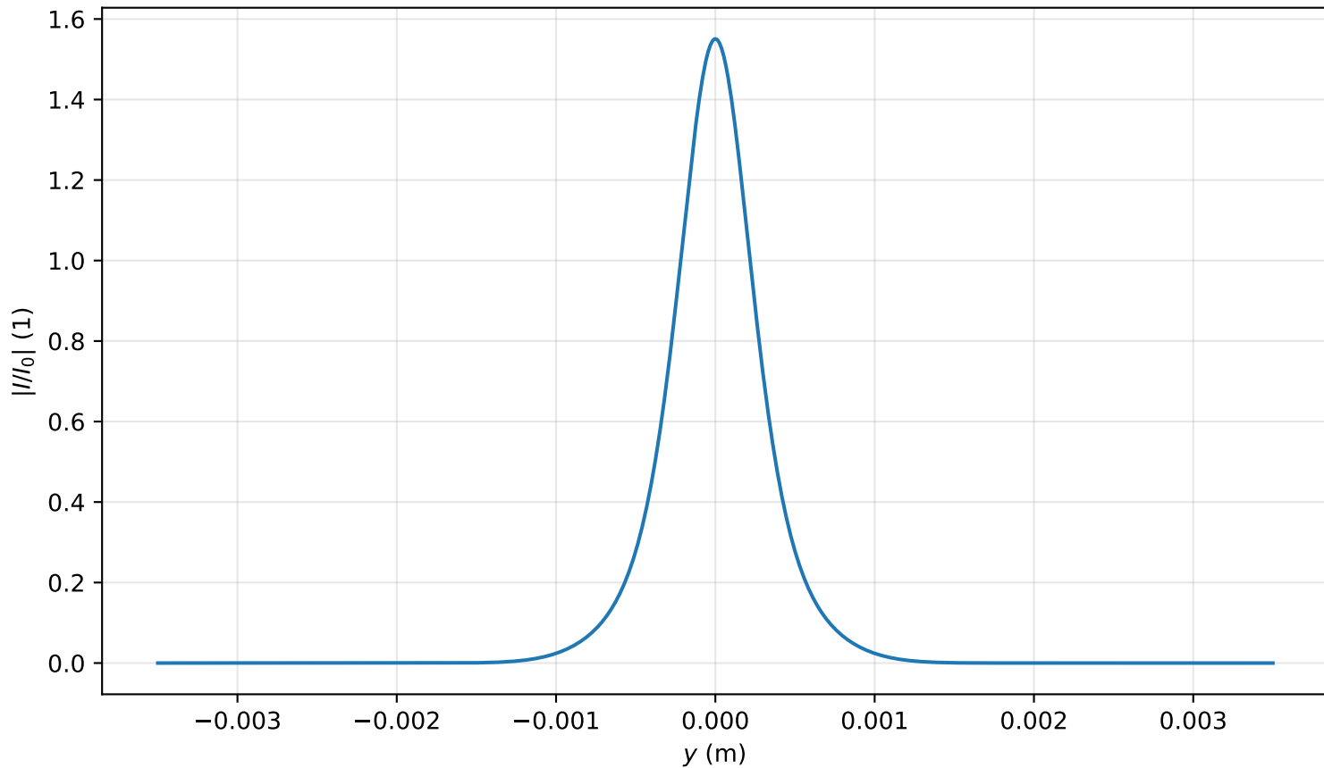
Intensity profile I(x=0, y, z=1.035)/I_0 , P_{in}=1.0P_{cr} , artificial time
